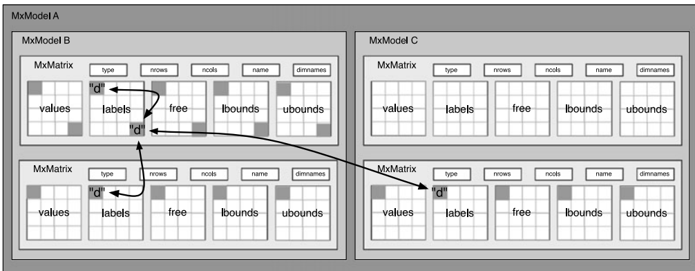
FIGURE 4. Equality constraints can be defined between submodels.
