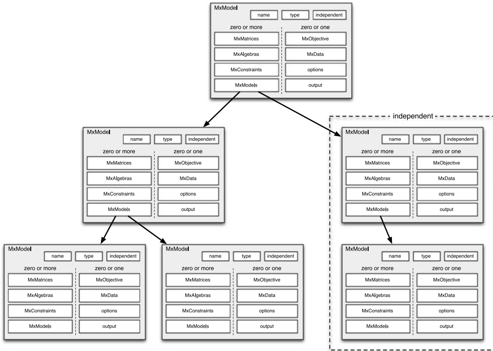
FIGURE 3. MxModels can contain lists of submodels.
