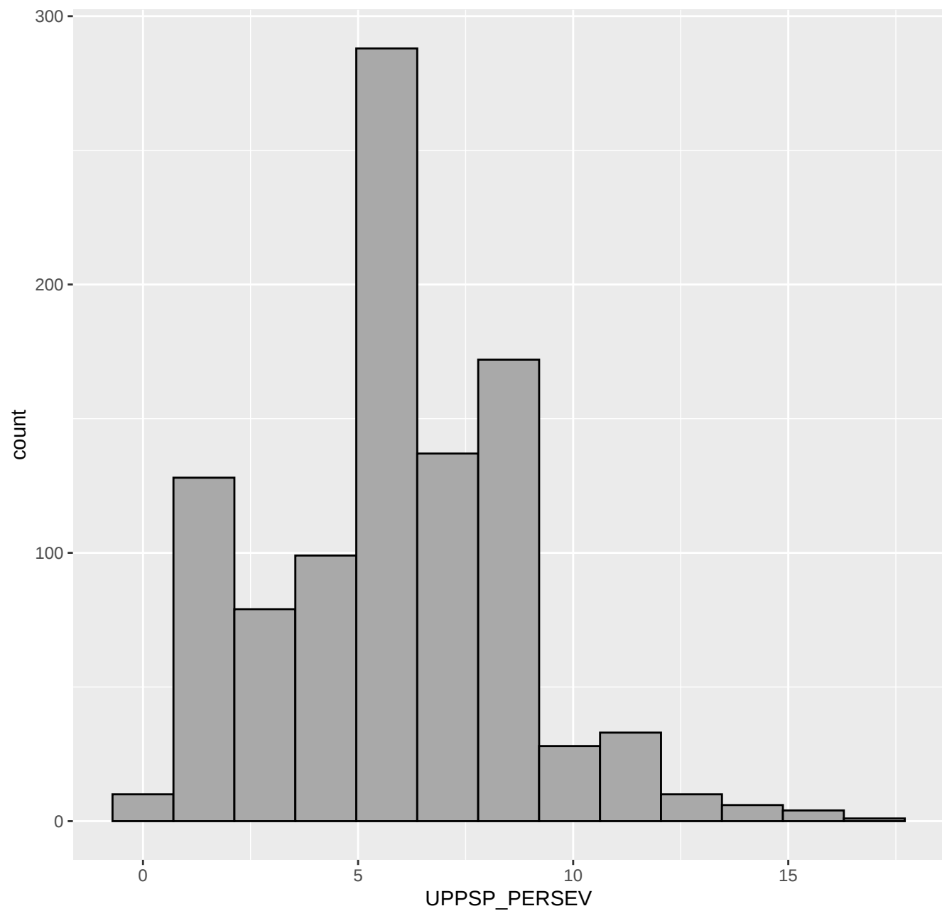
UPPS_Lack of Perseveration Score
