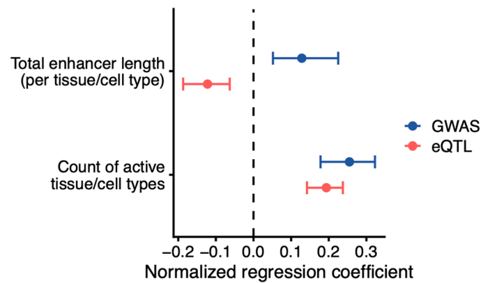
Extended Data Fig. 4 | GWAS and eQTL genes have different enhancer architectures. Same as Fig. 3b, but using enhancer-gene links predicted by the activity-by-contact (ABC) model from Nasser et al. 51 (Methods). For a given gene, we computed (i) the number of biosamples in which a gene has an enhancer, and (ii) the average total enhancer length (in base pairs) across active biosamples.
