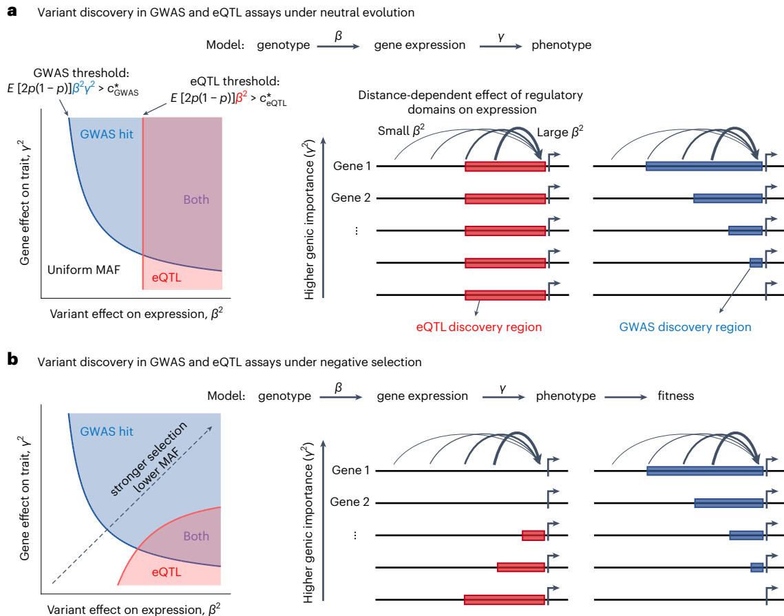
Fig. 6 | A model for variant discovery in GWAS and eQTL assays. a , Case of a neutrally evolving phenotype. (Left) Variant discovery in the space defined by variant effect on expression, \beta , and genic effect on phenotype, \gamma . Shading colors represent parameter space for the discovery of GWAS hit only (blue), eQTL only (red) and both types (purple), determined conditional on E[2p(1-p)] which is independent of the effect sizes in the neutral case. (Right) Schematic of variant discovery mapped to cis -regulatory domains as a function of genic
