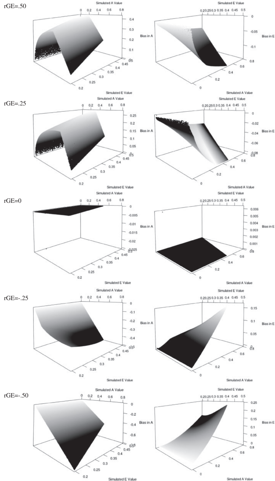
Fig. 3 Biases in A and E estimates as a function for gene-environment correlation.
