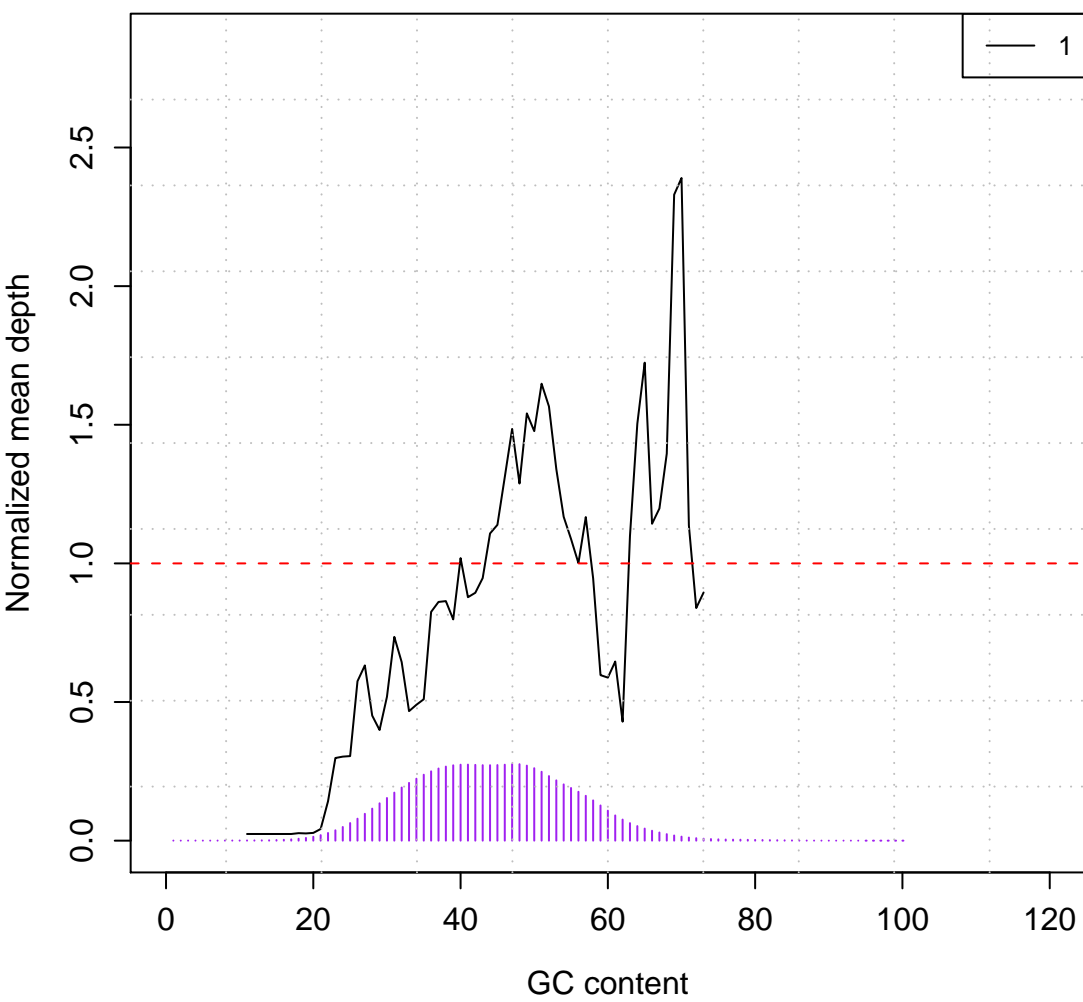
Mean depth vs. GC
