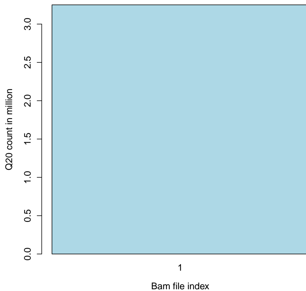
Empirical Q20 count
