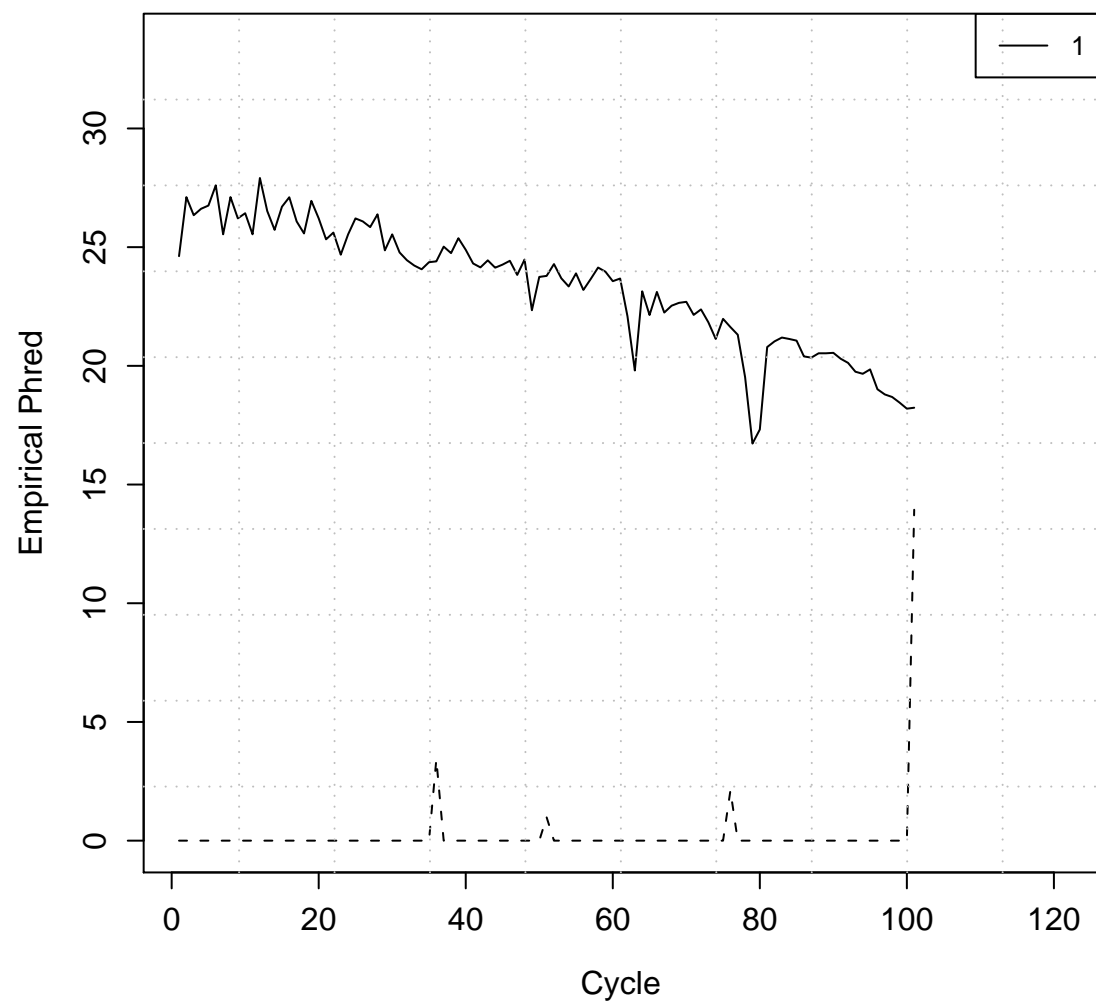
Empirical Phred score by cycle
