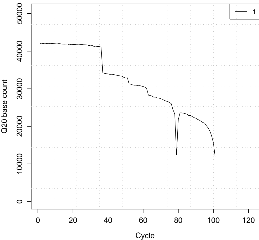
Q20 base count by cycle
