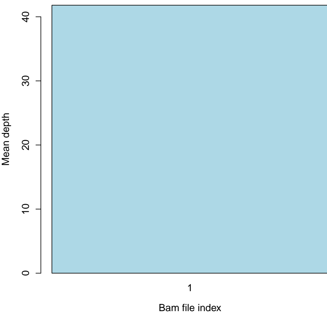
Mean depth of sequencing
