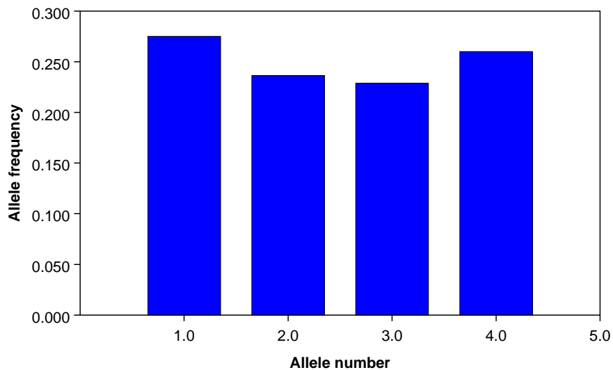
Overall distribution
