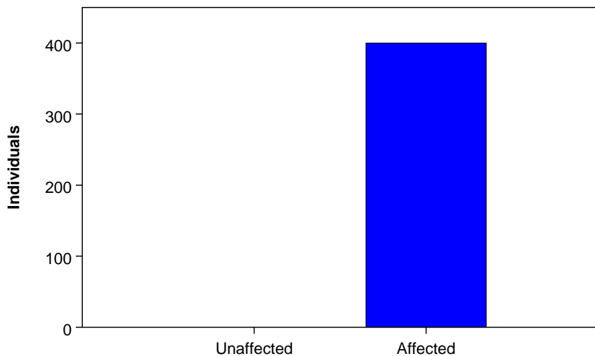
Overall distribution
