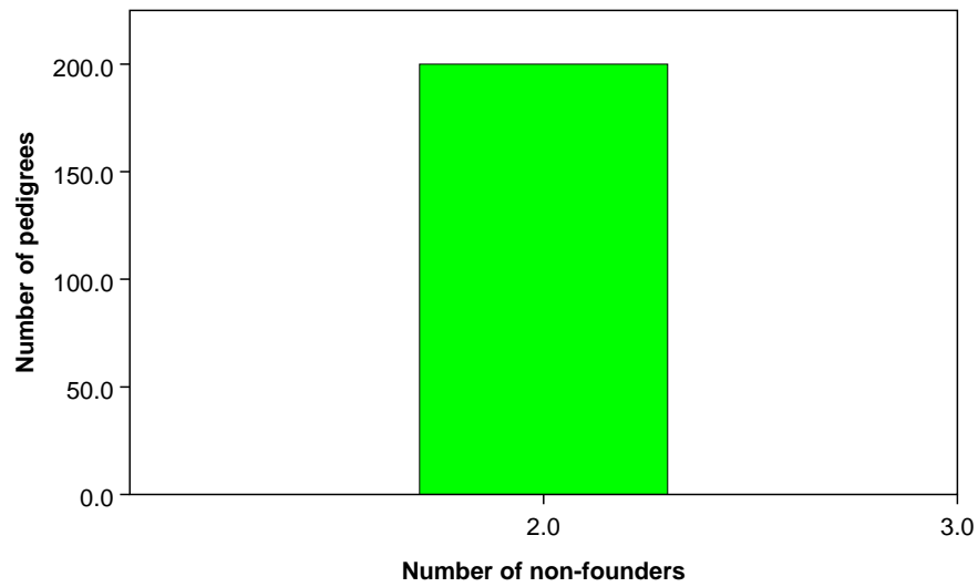
Non-founders
