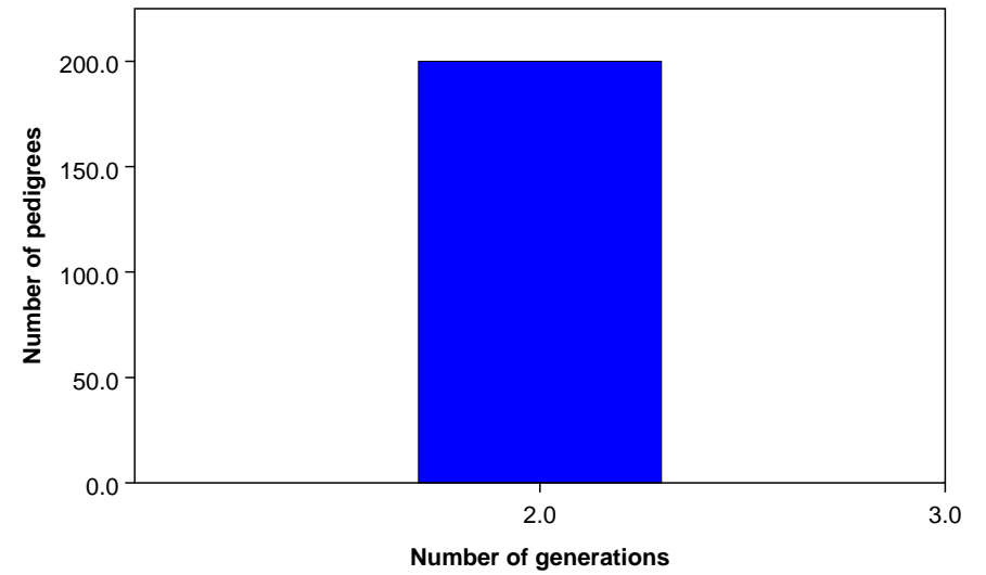
Generations
