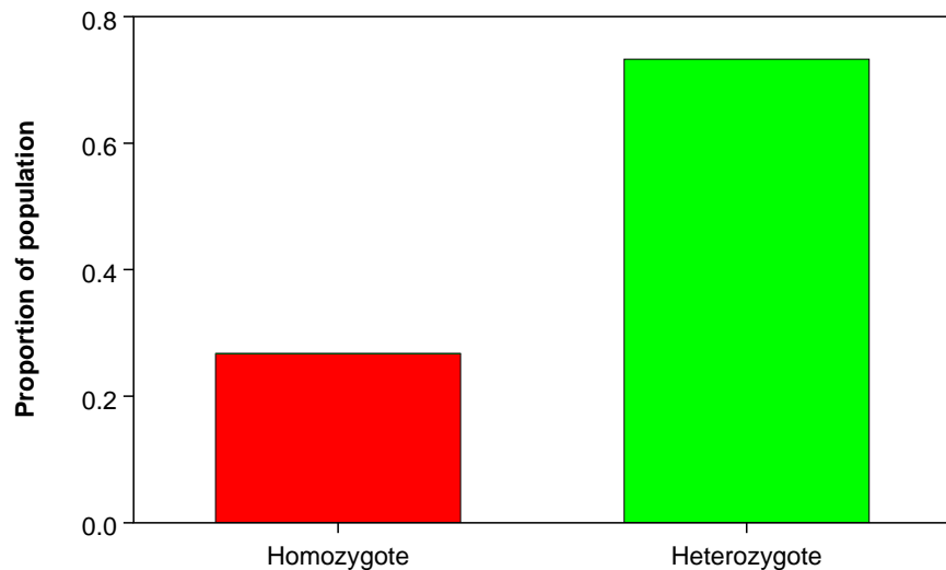
Informativeness
