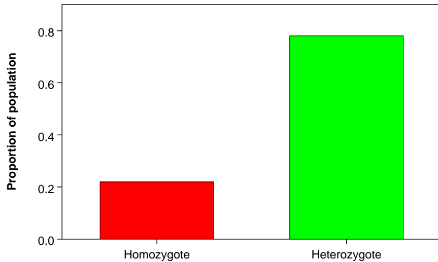
Informativeness
