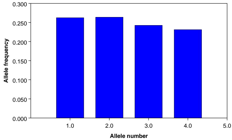
Overall distribution
