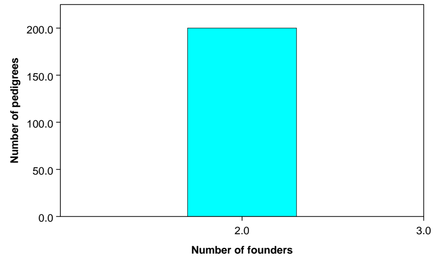
Founders
