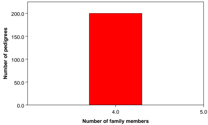
Individuals
