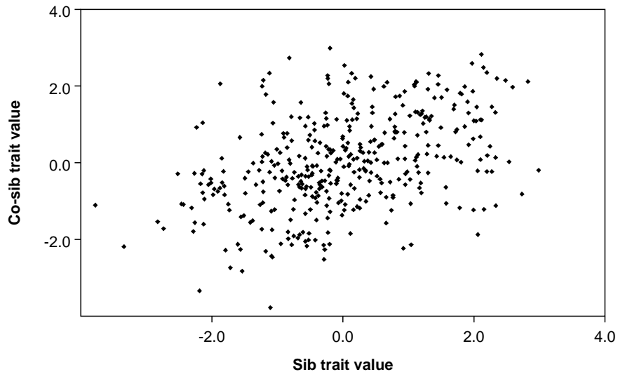
Sib-sib plot
