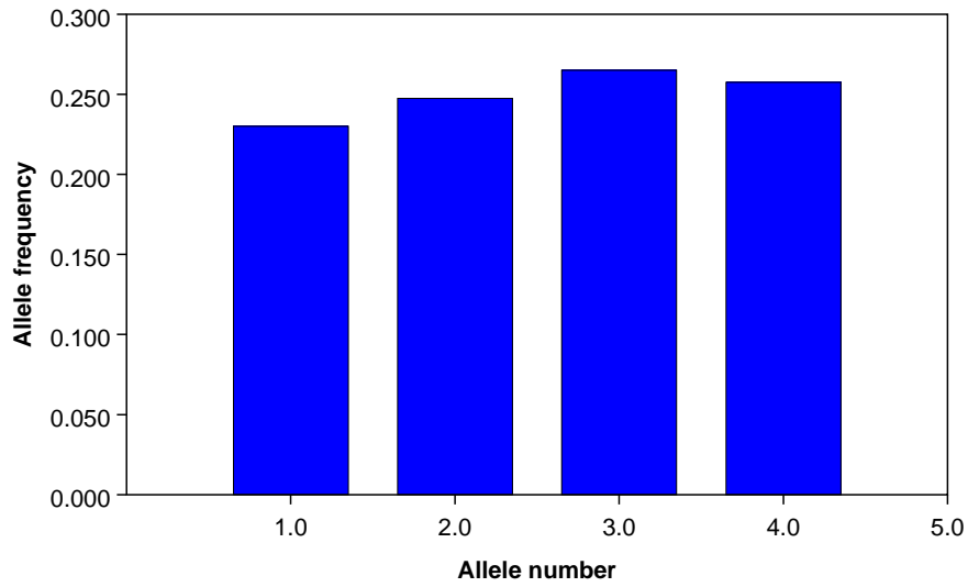
Overall distribution
