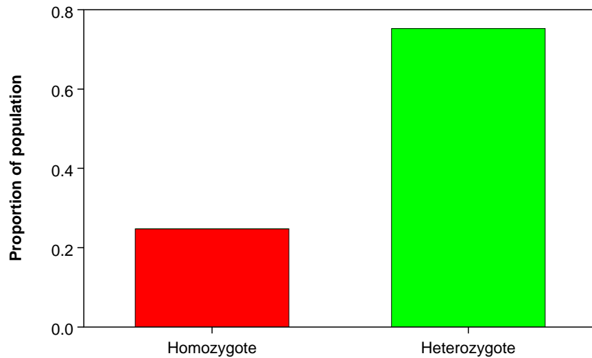
Informativeness
