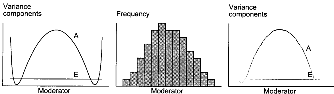
Figure 7 Visualization of variance components for the nonlinear G \times E example.
